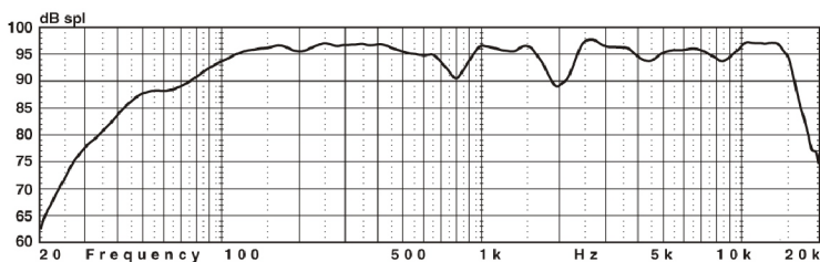
on axis response (2.83v@1m, free-field conditions)
